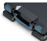
O&O BlueCon
