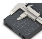
O&O DiskStat
